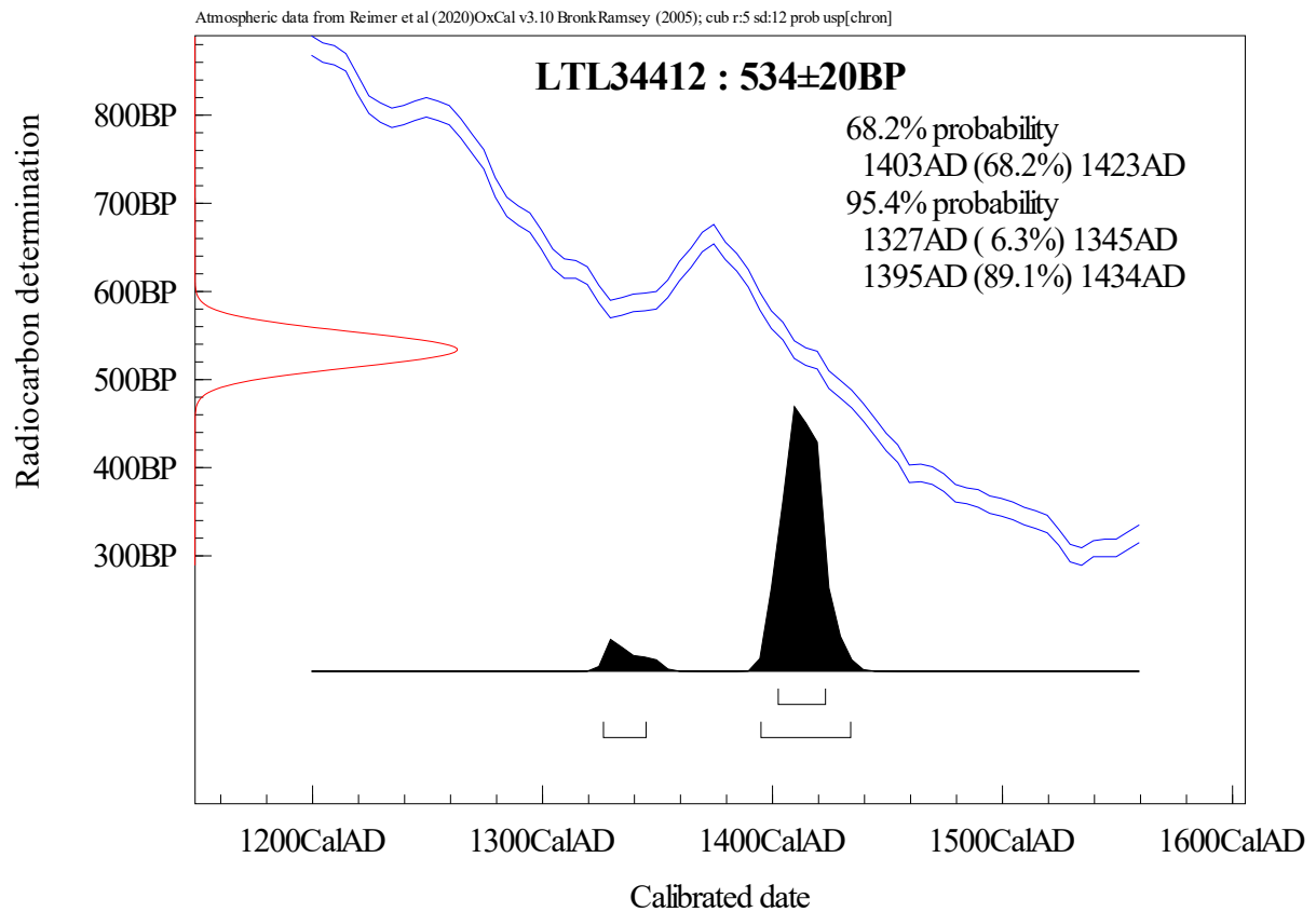
Figure 1. Calibration of the radiocarbon age of the sample LTL34412.
