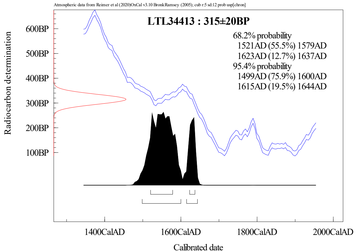
Figure 2. Calibration of the radiocarbon age of the sample LTL34413.
