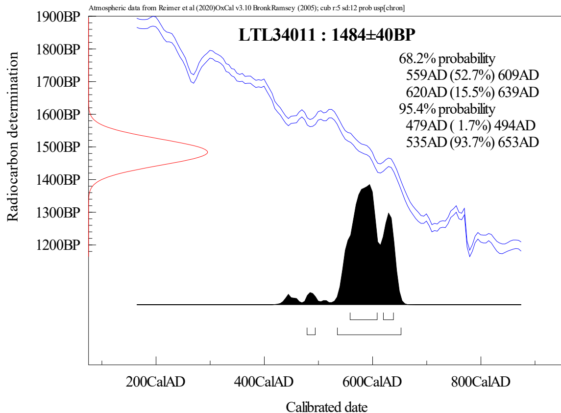
Figure 3. Calibration of the radiocarbon age of the sample LTL34011.
