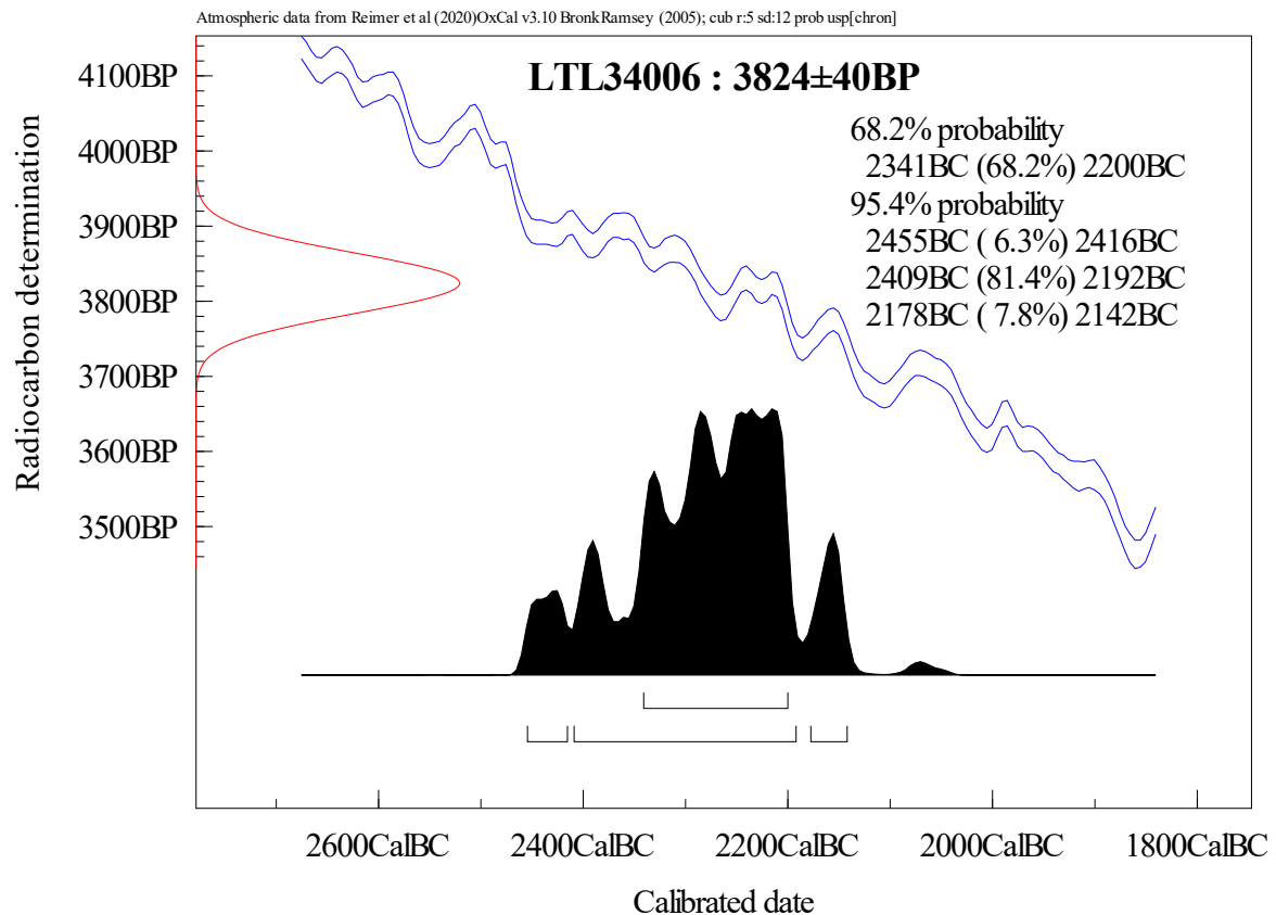
Figure 1. Calibration of the radiocarbon age of the sample LTL34006.
