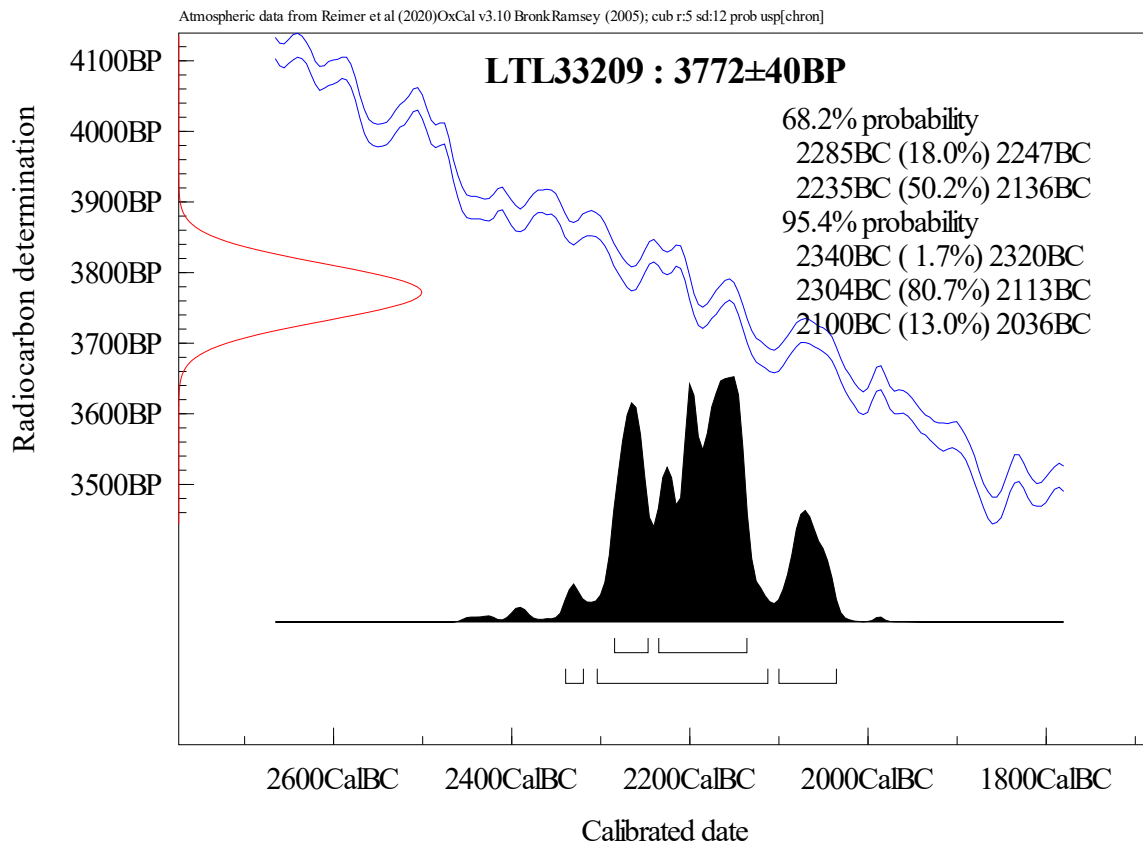
Figure 2. Calibration of the radiocarbon age of the sample LTL33209.
