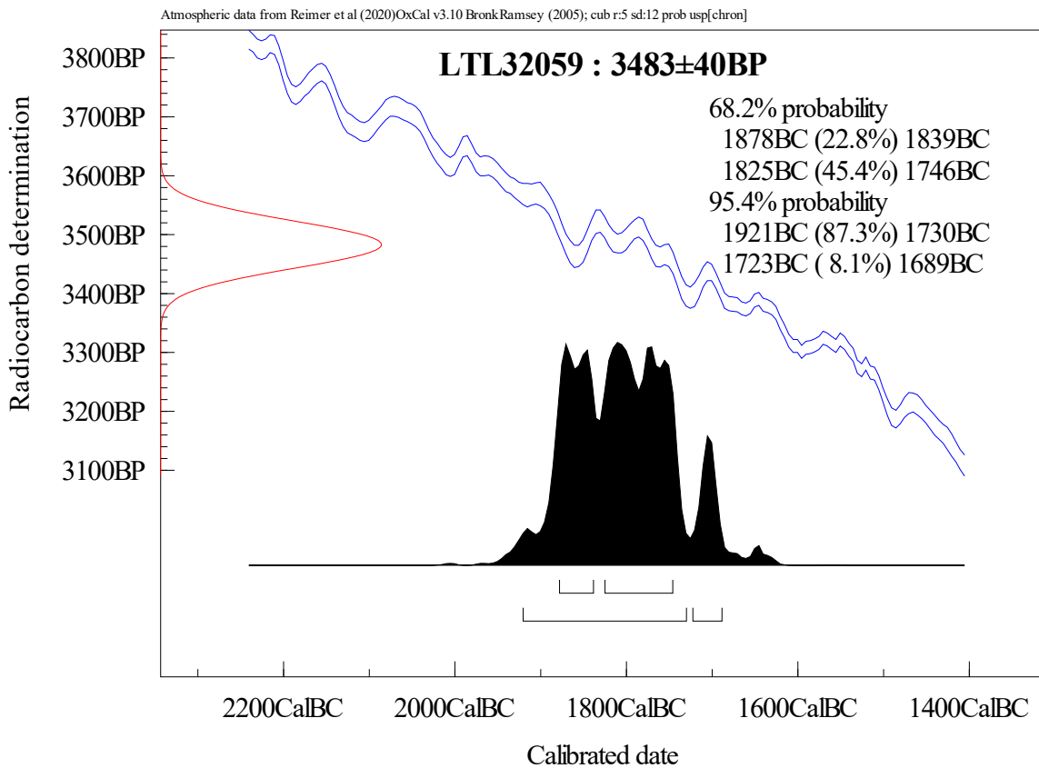
Figure 5. Calibration of the radiocarbon age of the sample LTL32059.
