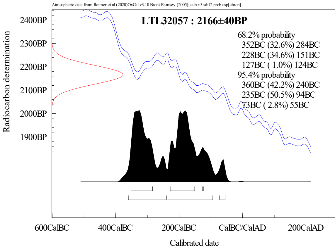
Figure 3. Calibration of the radiocarbon age of the sample LTL32057.
