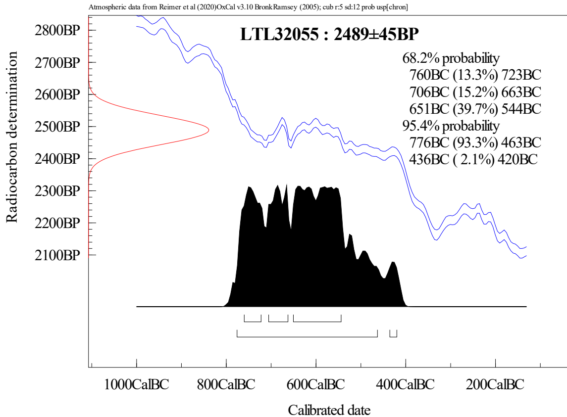
Figure 1. Calibration of the radiocarbon age of the sample LTL32055.
