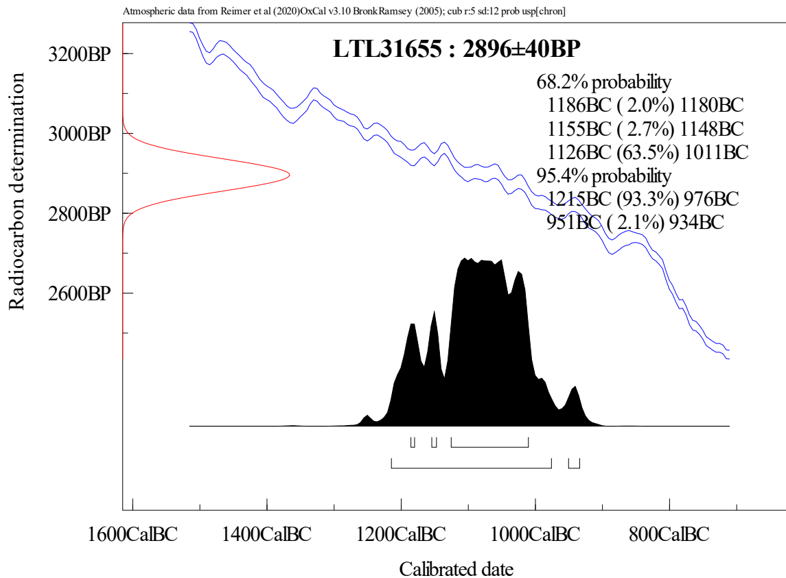
Figure 1. Calibration of the radiocarbon age of the sample LTL31655.
