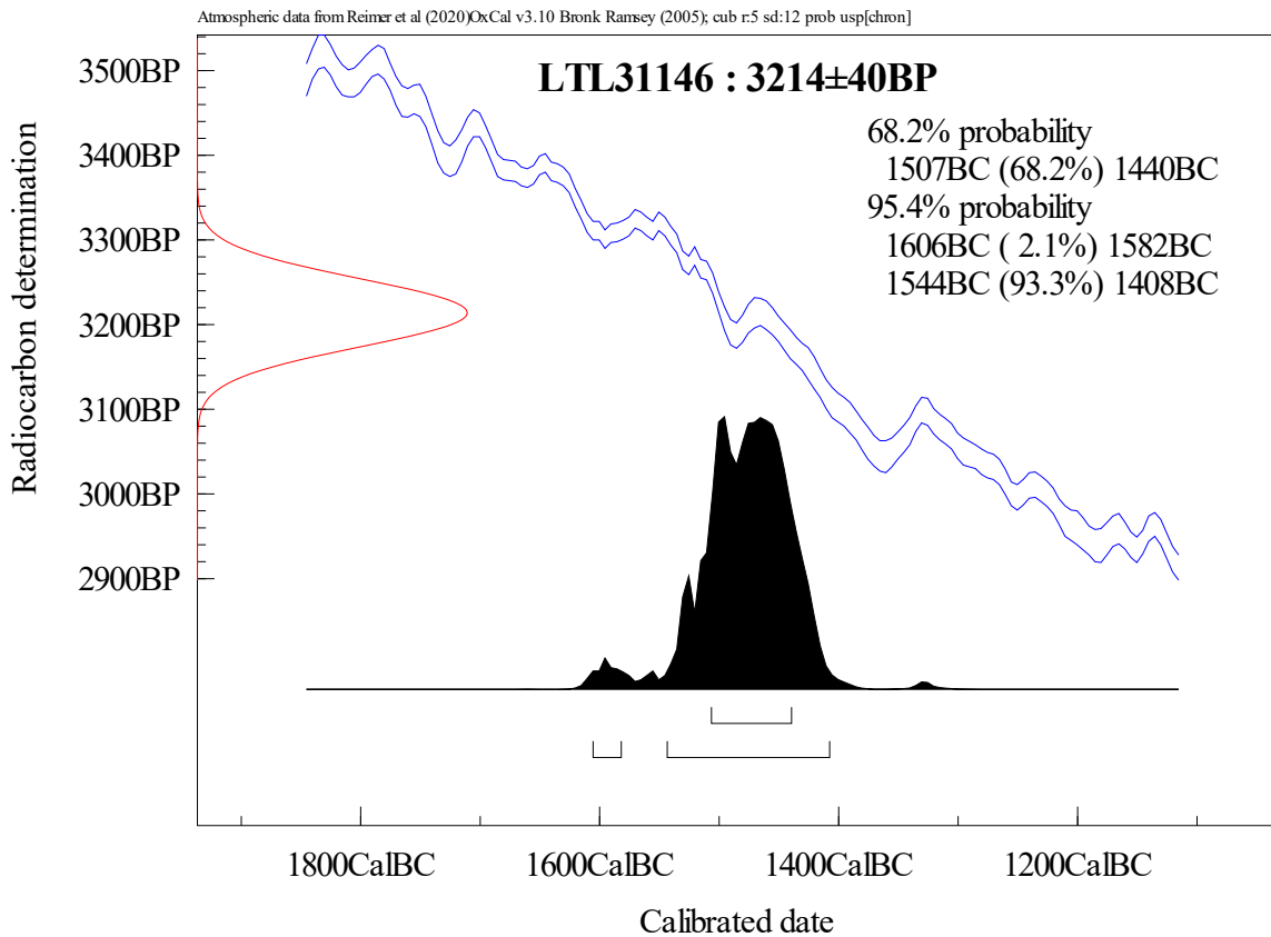
Figure 2. Calibration of the radiocarbon age of the sample LTL31146.
