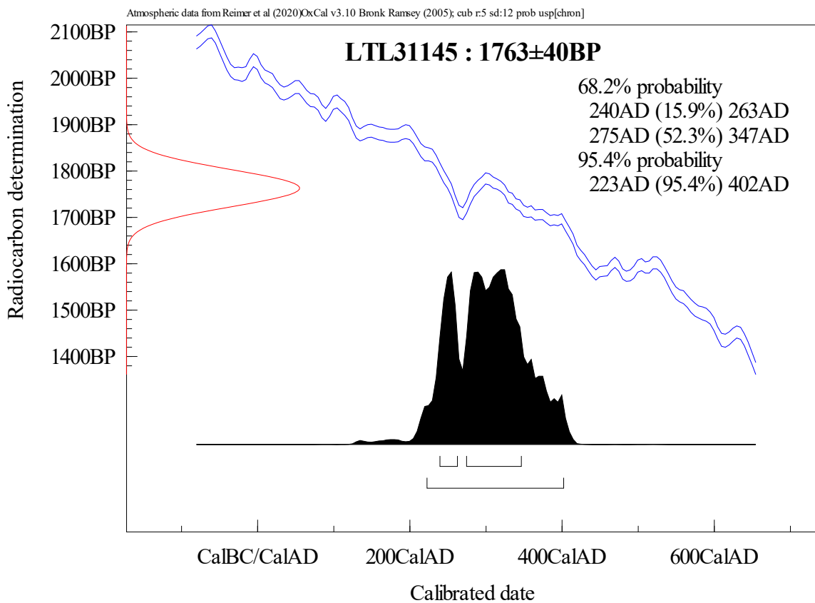
Figure 1. Calibration of the radiocarbon age of the sample LTL31145.
