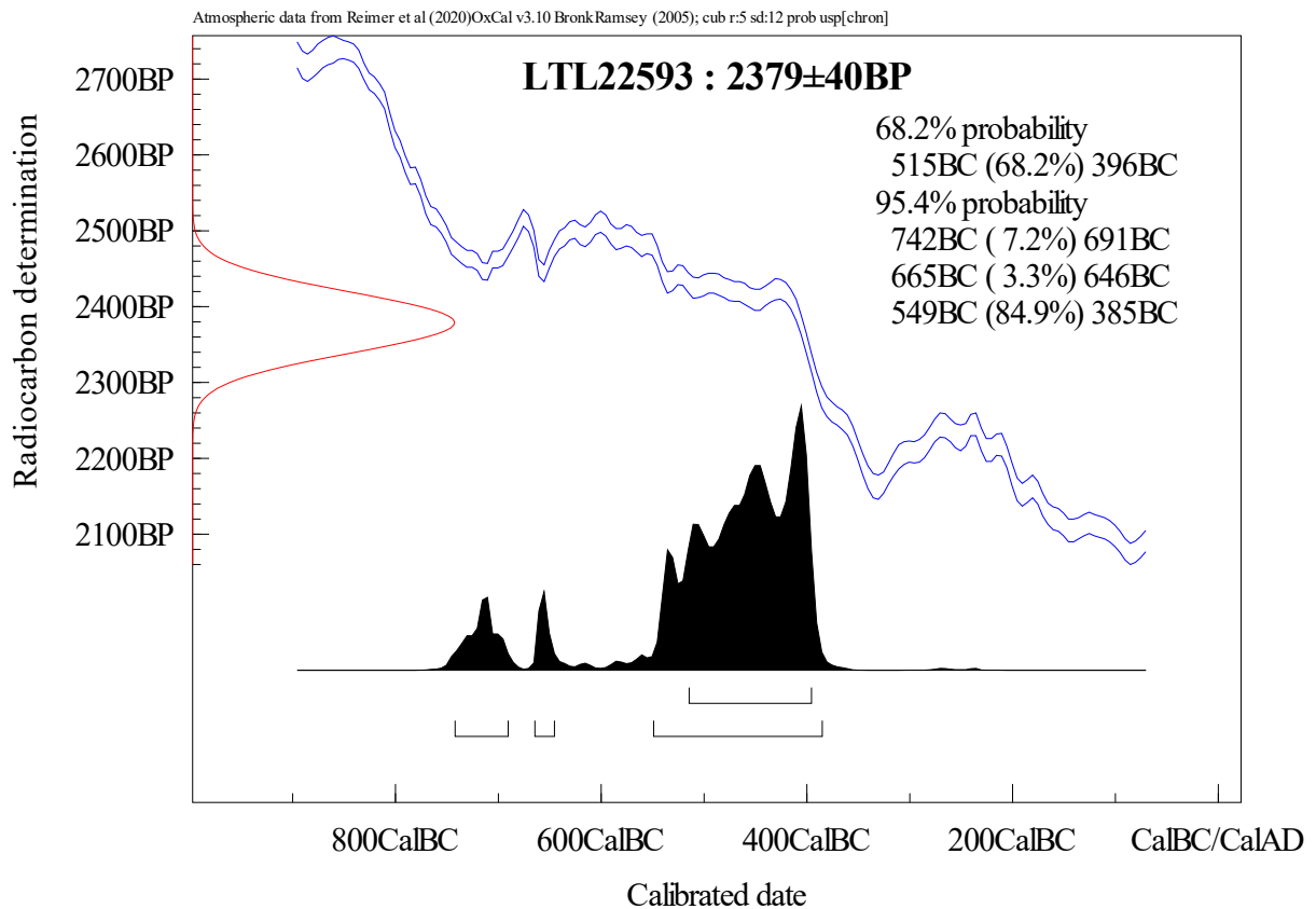
Figure 1. Calibration of the radiocarbon age of the sample LTL22593.
