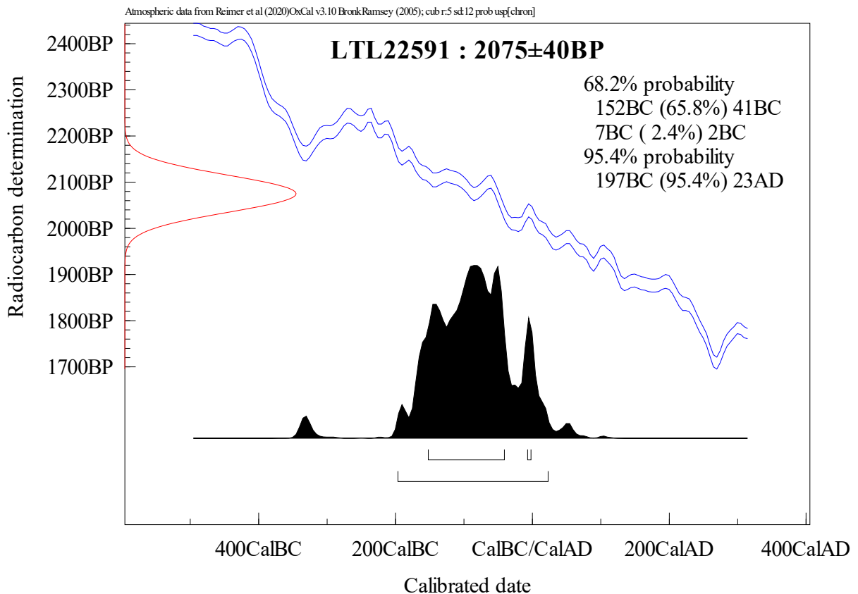
Figure 1. Calibration of the radiocarbon age of the sample LTL22591.
