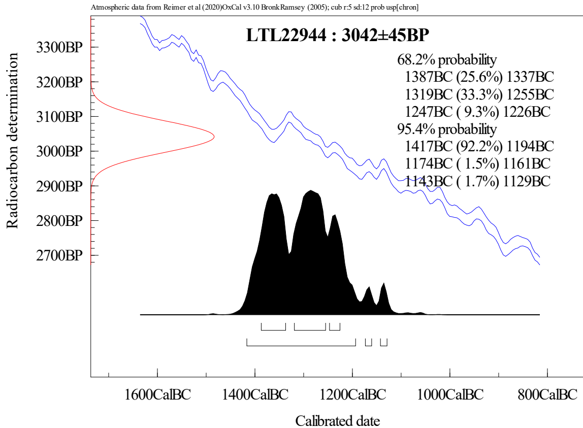
Figure 2. Calibration of the radiocarbon age of the sample LTL22944.
