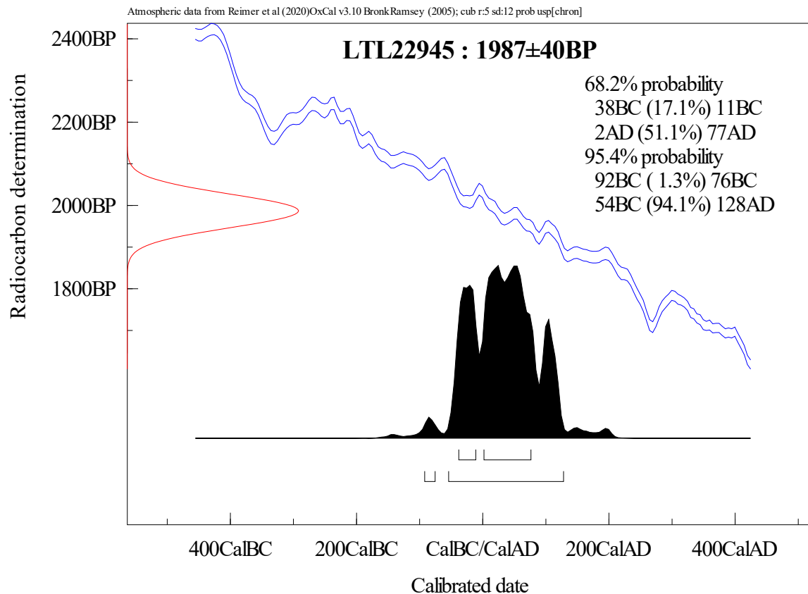
Figure 3. Calibration of the radiocarbon age of the sample LTL22945.
