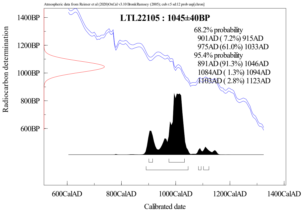
Figure 1. Calibration of the radiocarbon age of the sample LTL22105.
