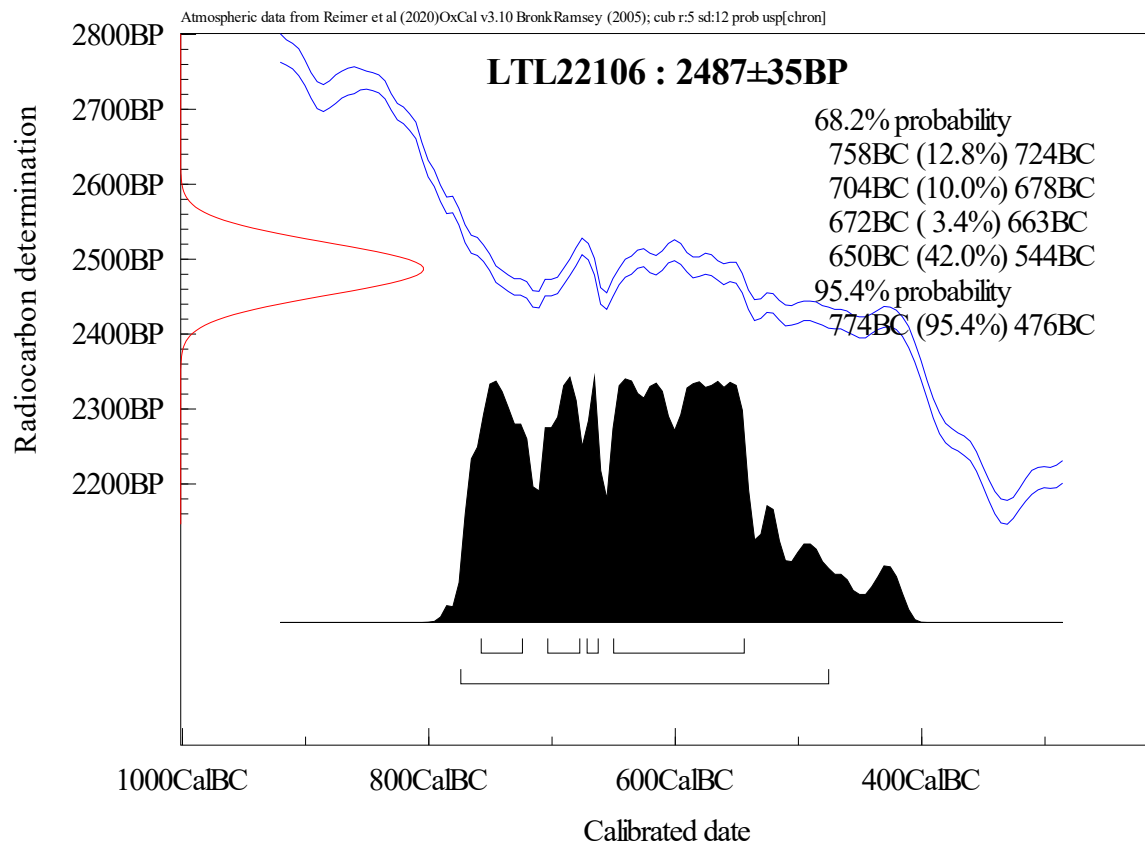
Figure 2. Calibration of the radiocarbon age of the sample LTL22106.
