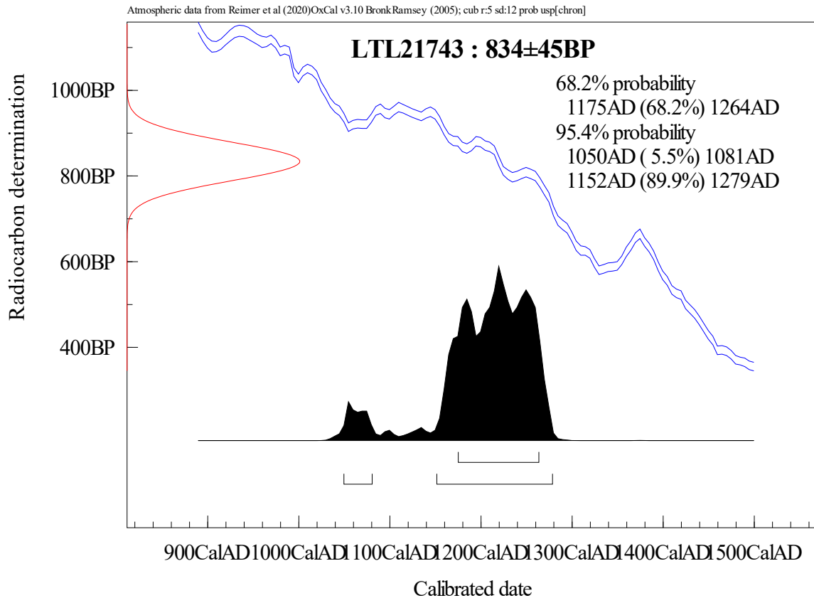
Figure 1. Calibration of the radiocarbon age of the sample LTL21743.
