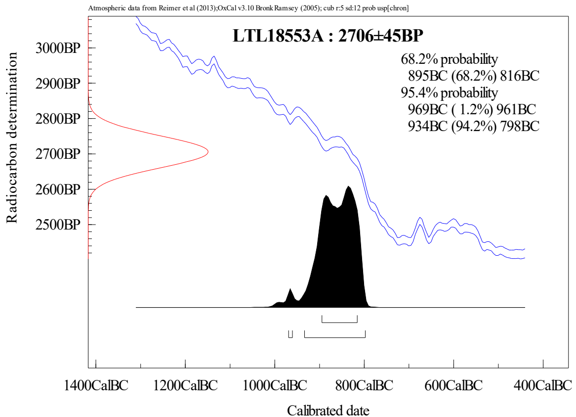
Figure 2. Calibration of the radiocarbon age of the sample LTL18553A.
