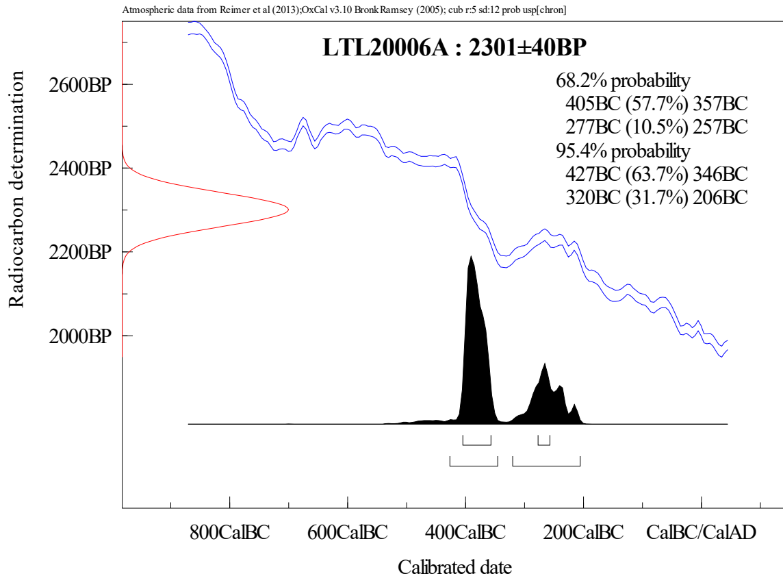
Figure 1. Calibration of the radiocarbon age of the sample LTL20006A.
