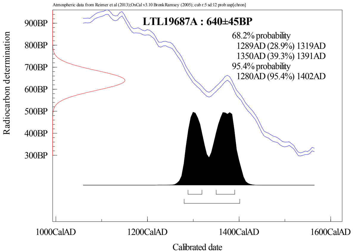
Figure 1. Calibration of the radiocarbon age of the sample LTL19687A.
