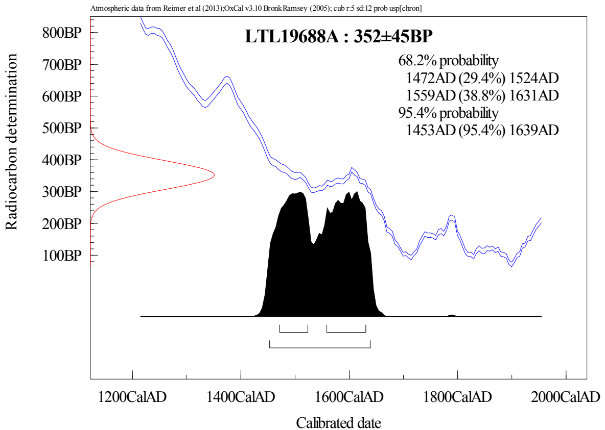
Figure 2. Calibration of the radiocarbon age of the sample LTL19688A.
