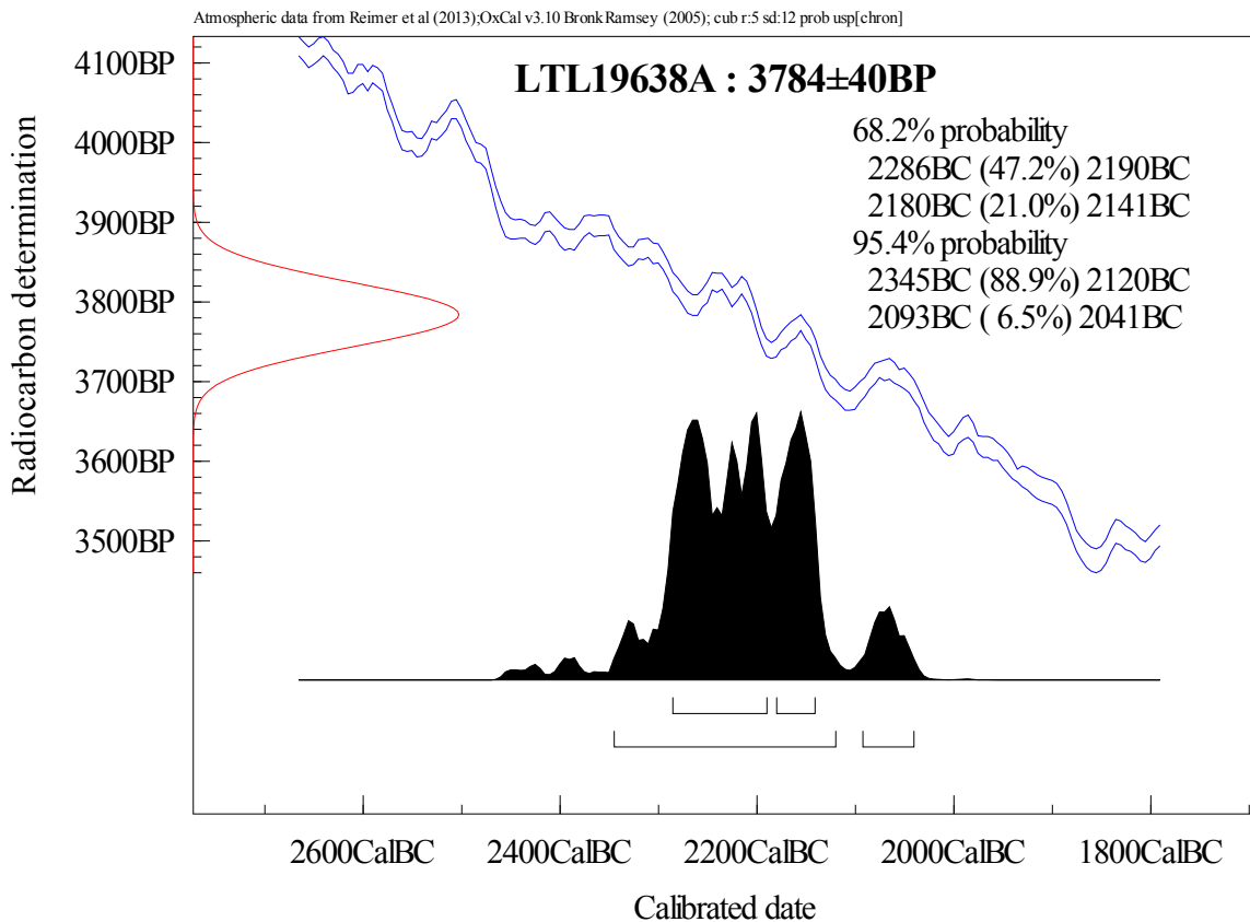
Figure 1. Calibration of the radiocarbon age of the sample LTL19638A.
